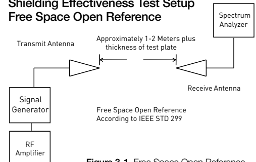
Figure 3-1. Free Space Open Reference
