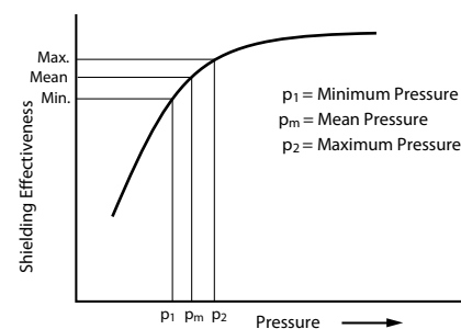
Figure 1-15. Typical Gasket Performance Curve
